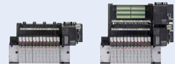
Type 8640 with 12x 2x3/2-way valves with Profibus DP (with 24 digital inputs – in picture at right)
